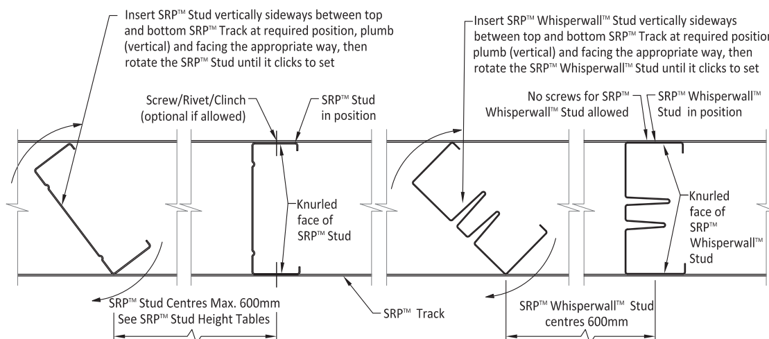
FIGURE 2 SRP™ Stud and SRP™ Whisperwall Installation
