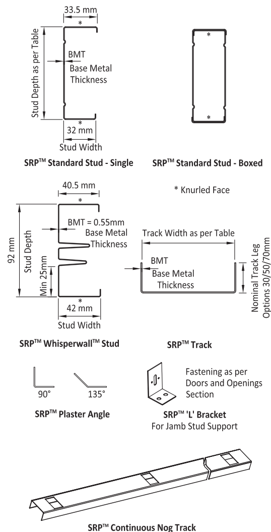
FIGURE 1 SRP™ Wall Product Range
